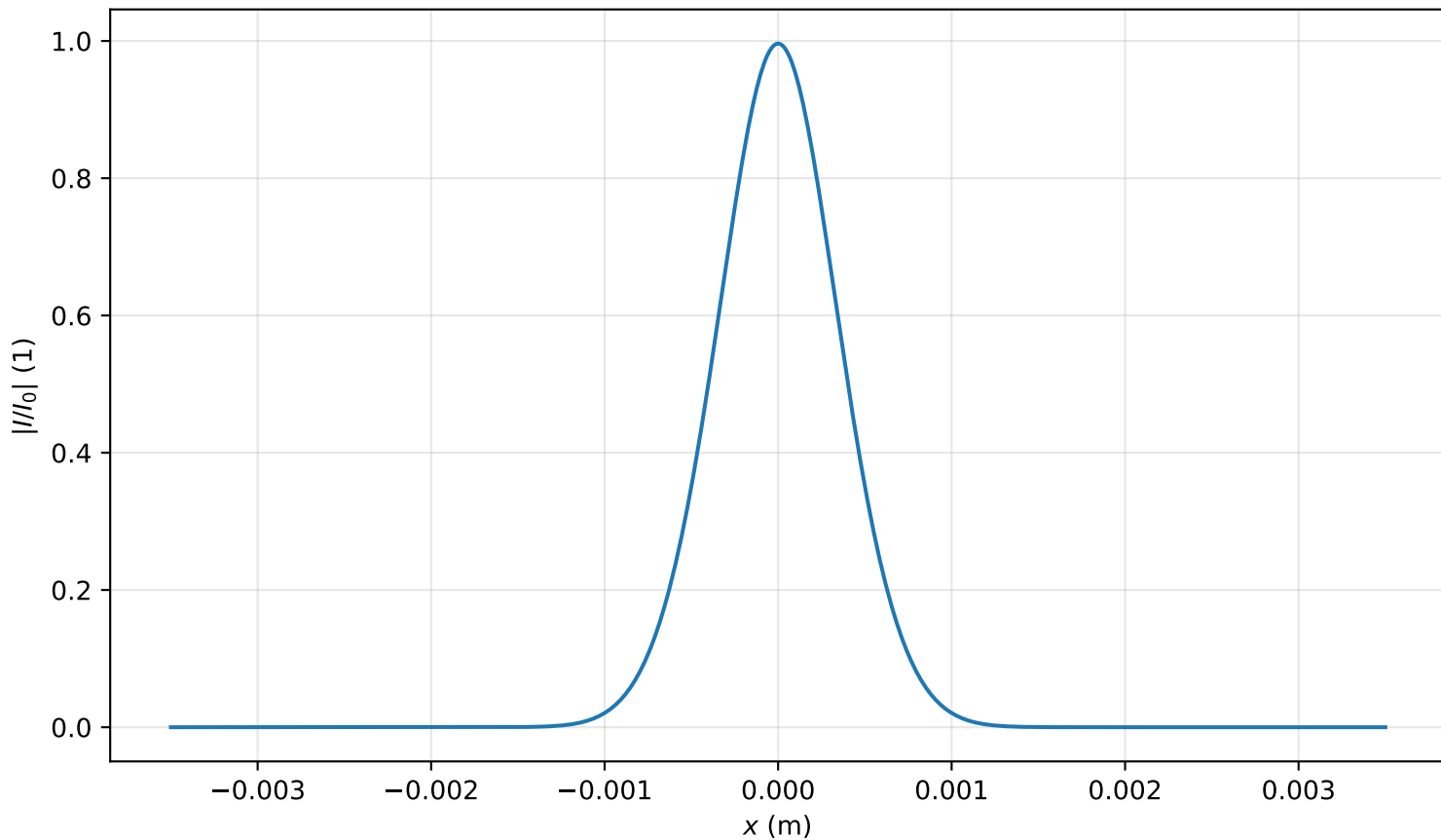
Intensity profile I(x, y = 0, z = 0.557m)/I_0 , P_{in}=0.3P_{cr} , artificial time
